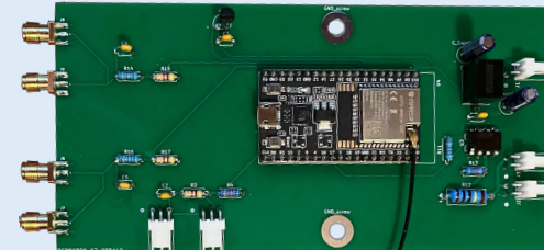
Figure 5: A picture of the PCB design of the Sensor Unit
