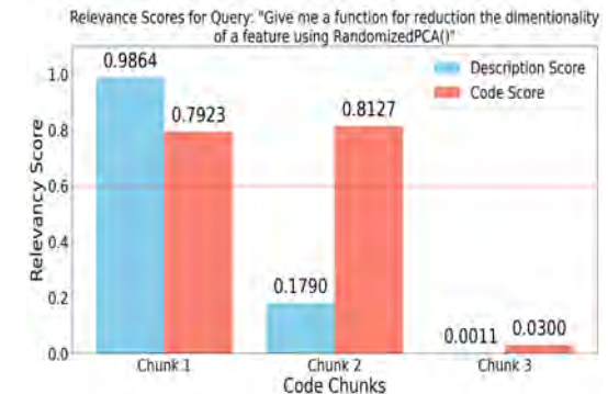
Figure 5: Comparison of scalar scores from description and code embeddings with cutoff line
