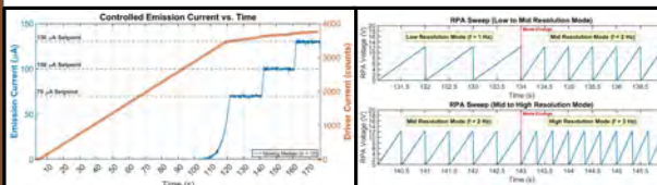
Fig. 5: Controlled emission current for 70, 100, and 130 \mu\text{A} setpoints
