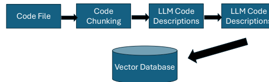
Figure 3: LLM Code Description Generation Pipeline
