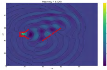
Figure 3: Simulation of a propagating EM sine wave reflecting of an angled dielectric screen in (V/m)
